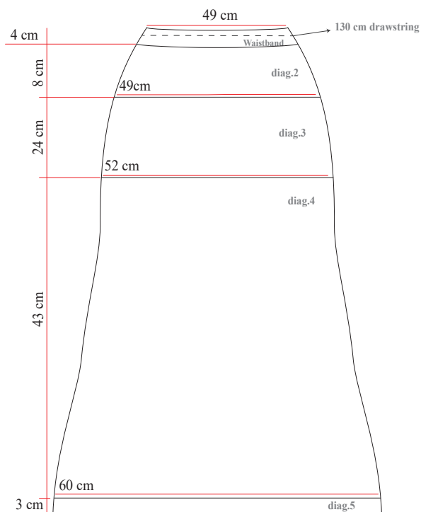
Measurement diagram
